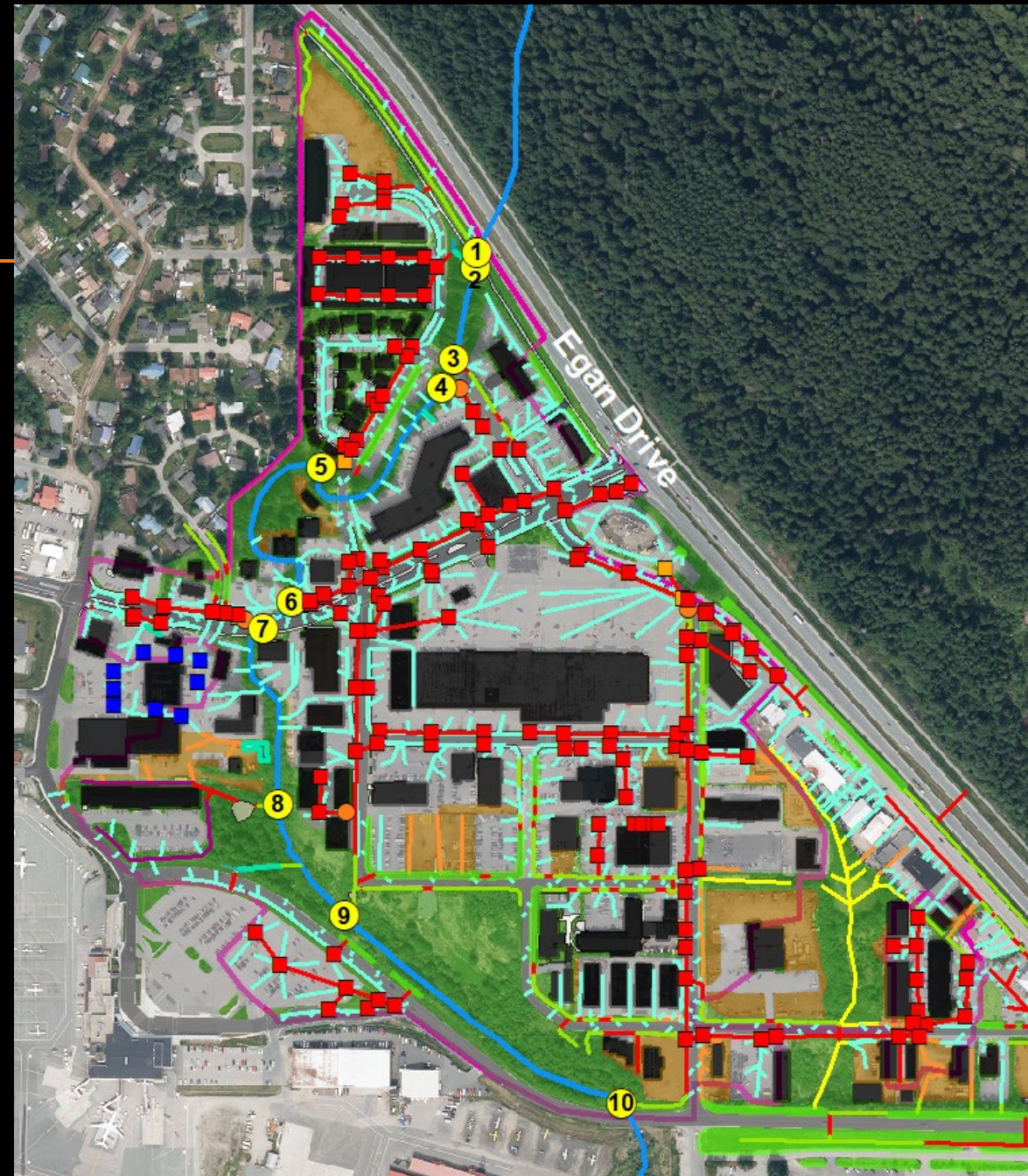
Lower Jordan Creek Stormwater System
