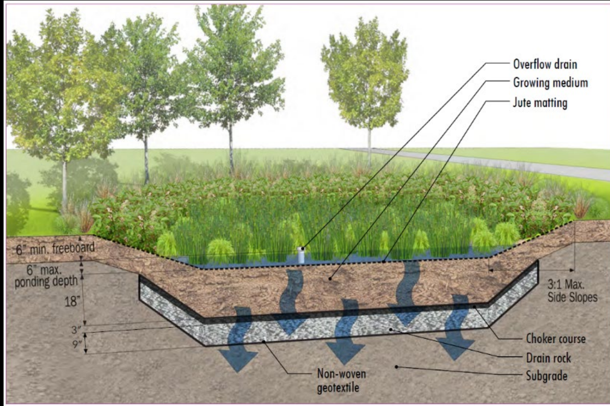
bioretention swale
