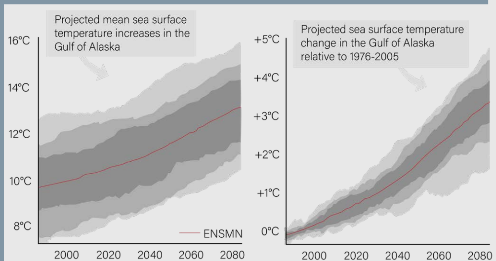
FIGURE 7. SEA SURFACE TEMPERATURES
