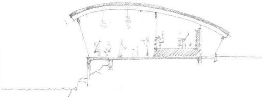
2 CONCEPTUAL - BUILDING SECTION
