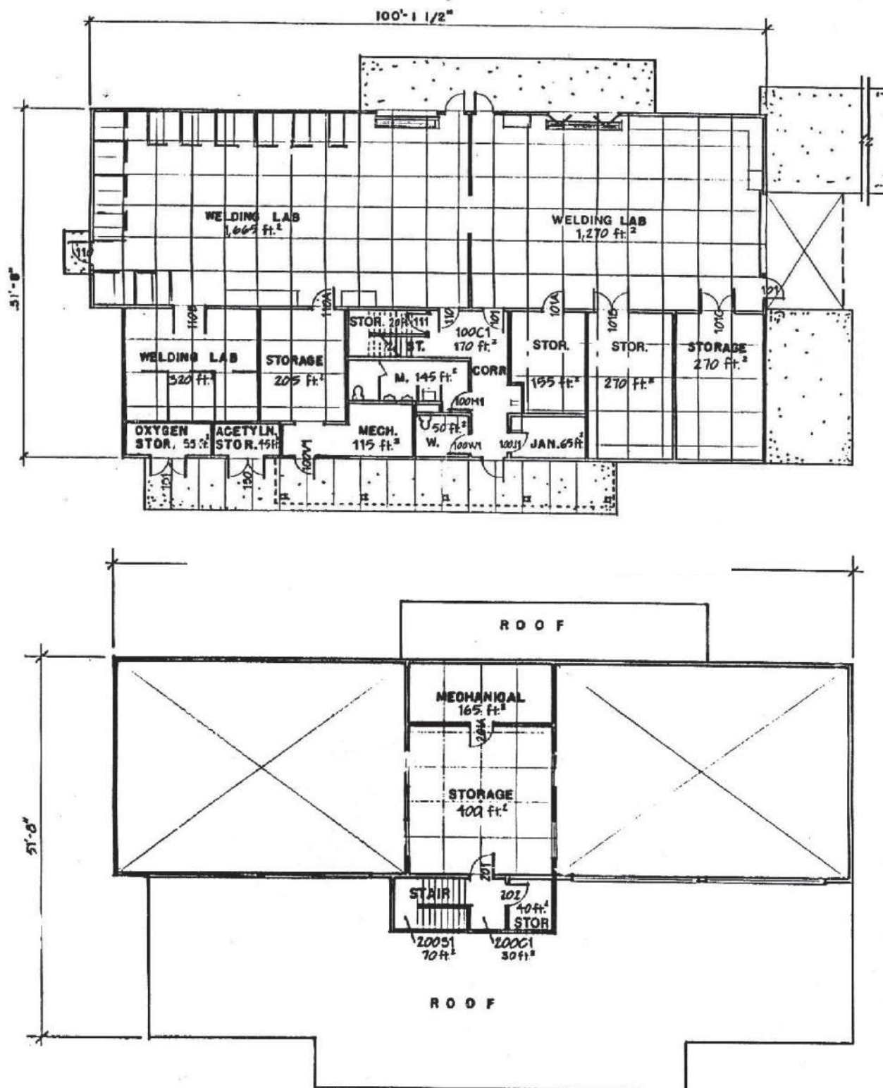
FIGURE 3.7 – Second floor layout of the Welding Lab
