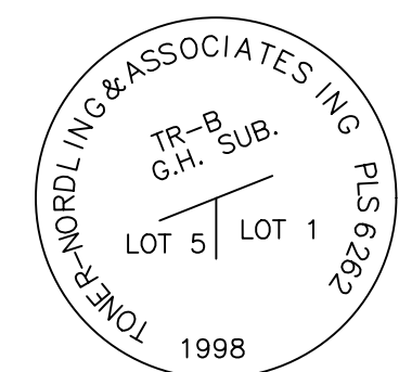
3" ALUMINUM MONUMENT DETAIL "A"
