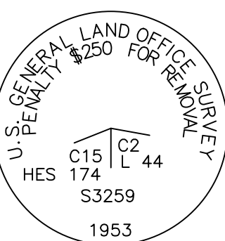
2" BRASS CAP DETAIL "C"
