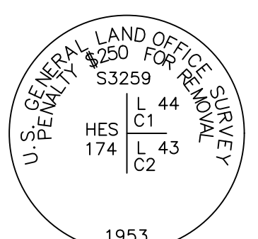
3" BRASS CAP DETAIL "E"
